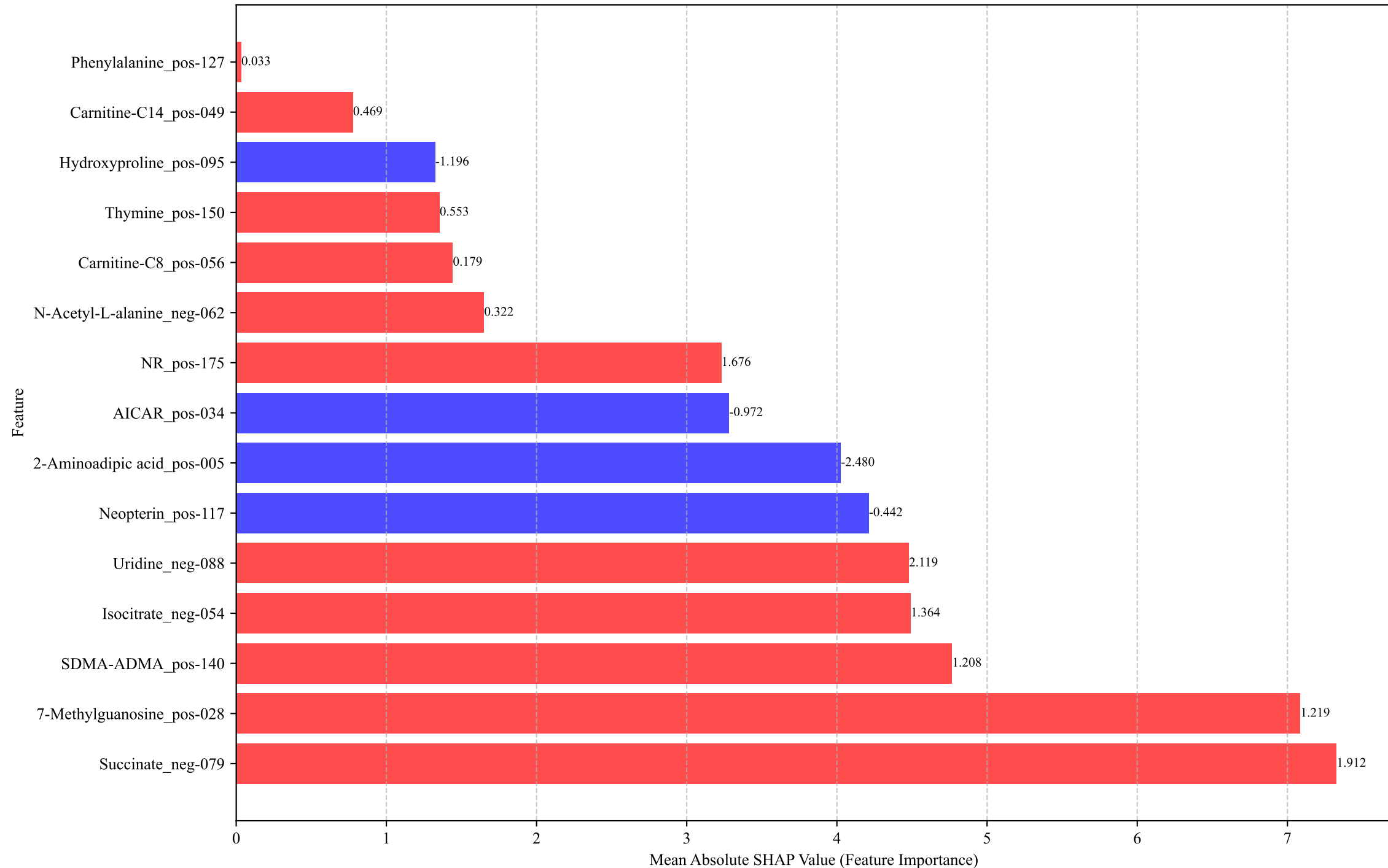
SHAP Analysis: Feature Importance and Risk Direction (Red: Risk Factor, Blue: Protective Factor)
